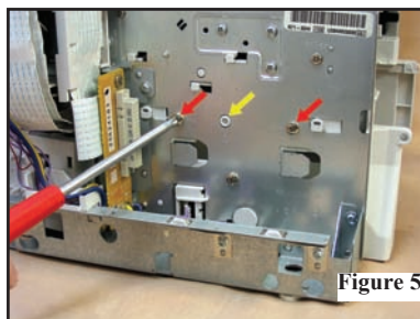
Figure 5 - Remove the two screws labeled "M4" (red arrows) and push the plastic circle (yellow arrow) to remove the right tray guide (Figure 6).
