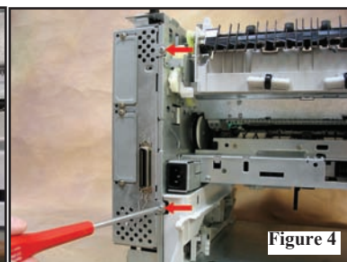
Figure 4 - The red arrows indicate the two screws that attach the formatter and its cage to the printer.
