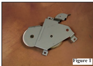
Figure 1 - The swing plate assembly for the HP LaserJet 4200/4300 series (part # RM1-0043).
