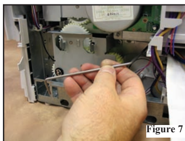
Figure 7 - Remove the switch rod.
