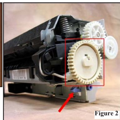
Figure 2 - The 4200/4300 series fuser has a 40-tooth gear (red box) that engages with the swing plate assembly. Blue clips on either side of the fuser (red arrow shows right clip) secure the fuser in the printer.
