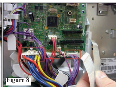
Figure 8 - The two white ribbon cables (being held) and three multi-colored cables (red boxes) must be removed from the DC controller.
